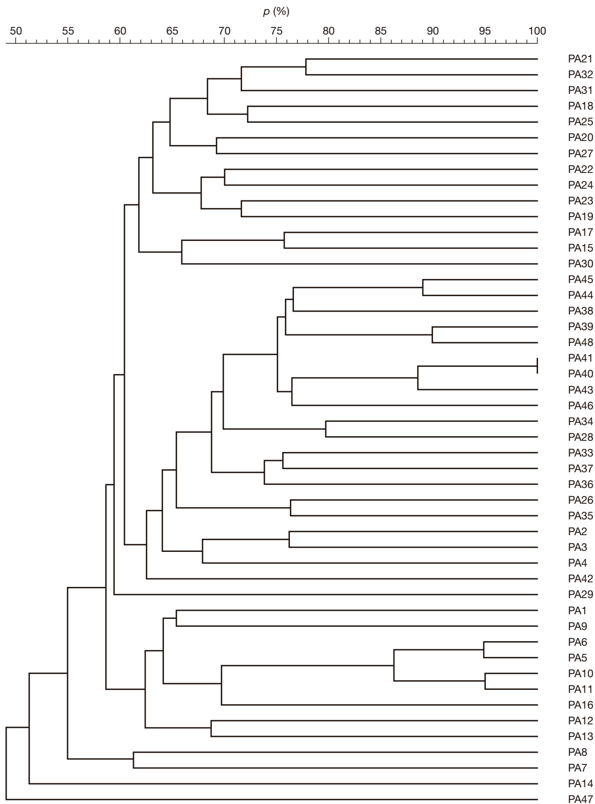
Fig. 1. Computed dendrogram derived from combined data analysis of enterobacterial repetitive intergenic consensus polymerase chain reaction, repetitive extragenic palindrome polymerase chain reaction, and pulsed-field gel electrophoresis patterns for 48 Pseudomonas aeruginosa isolates.
